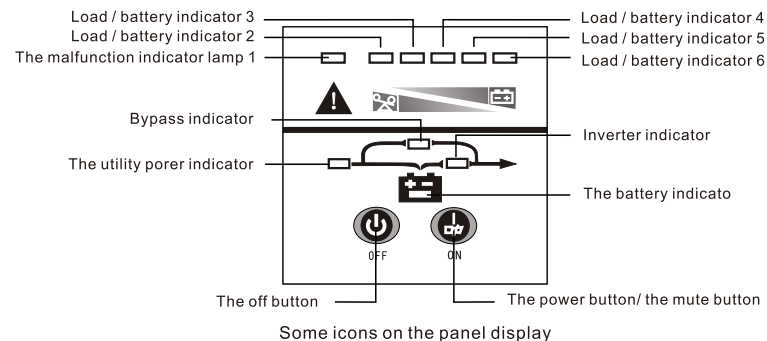
Some icons on the panel display
