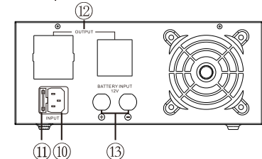
Back panel
