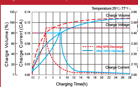
Charge Characteristic Curve for Cycle Use(IU)
